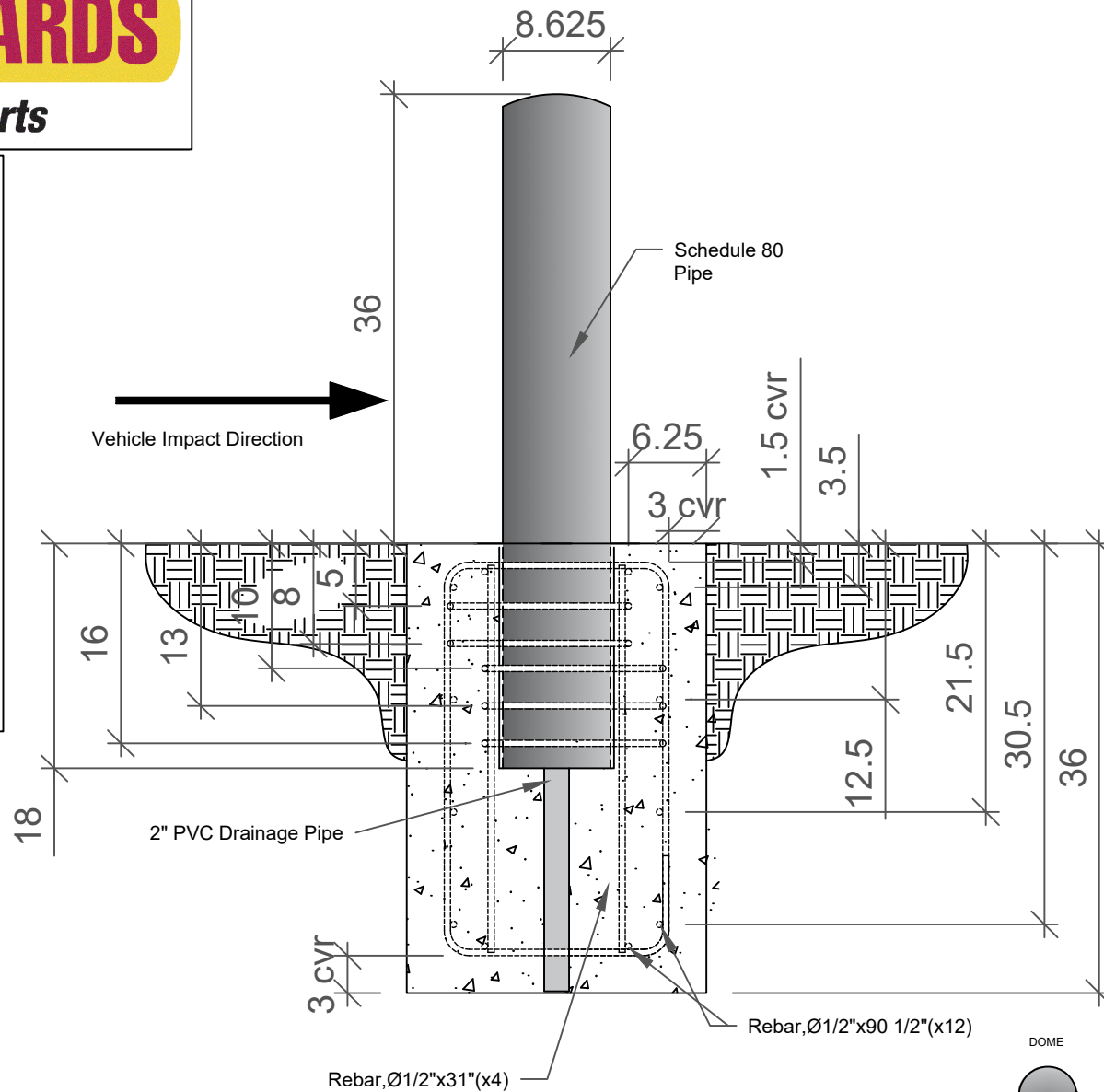
END VIEW-FOUNDATION
